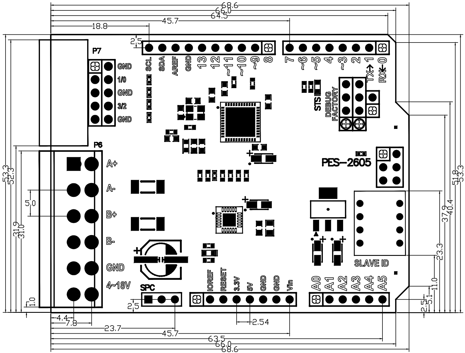
PES-2605 Dimension (mm)
